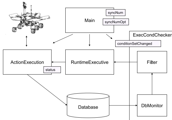
Figure 10: The K9 Executive and 4 of its 68 unprotected fields
