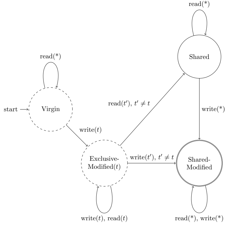
(a) ERASER state machine
